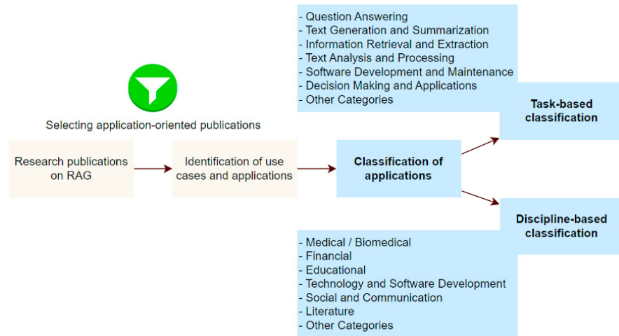
Fig. 2. Research Method
